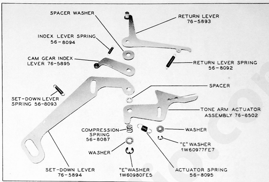
Figure 8. Actuator Assembly
