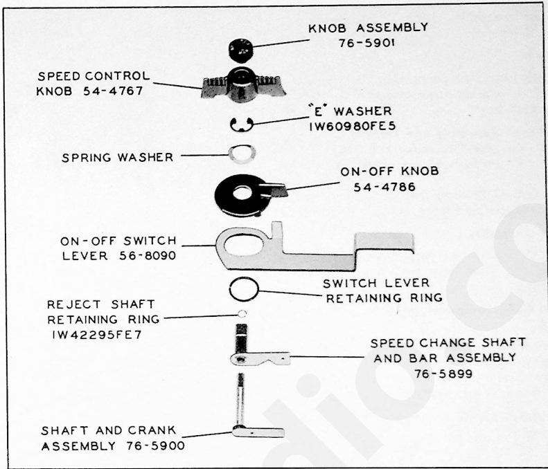
Figure 10 Control Assembly
