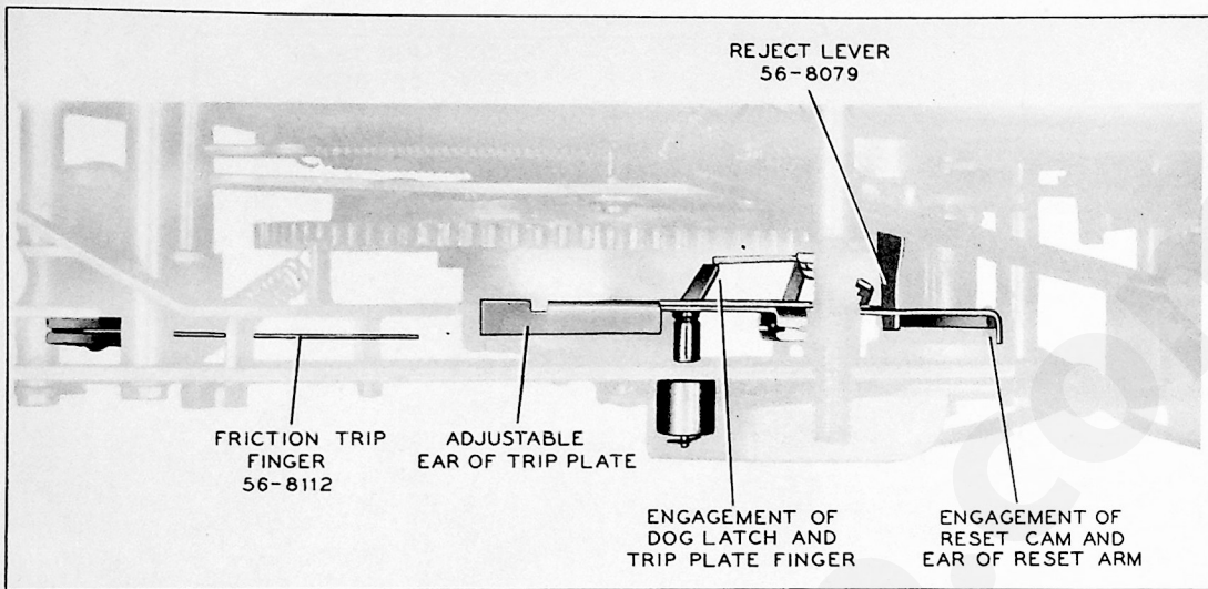
Figure 4. Trip Adjustment
