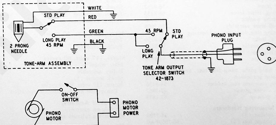
Figure 17. Wiring Diagram of Model M-22
