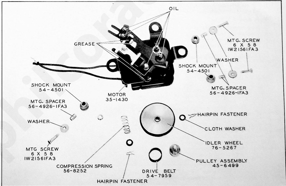
Figure 11. Motor Assembly—Part No. 35-1451
