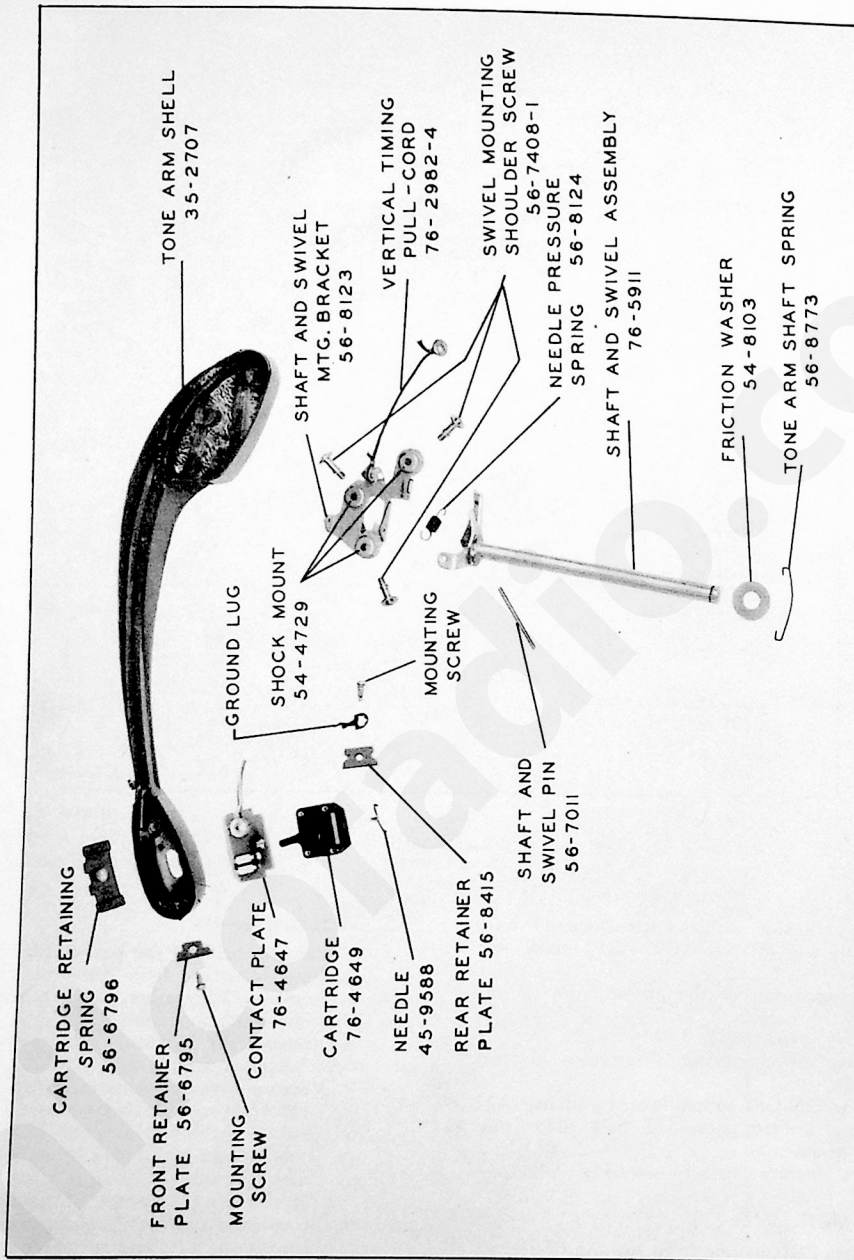
Figure 15. Tone-Arm Assembly
