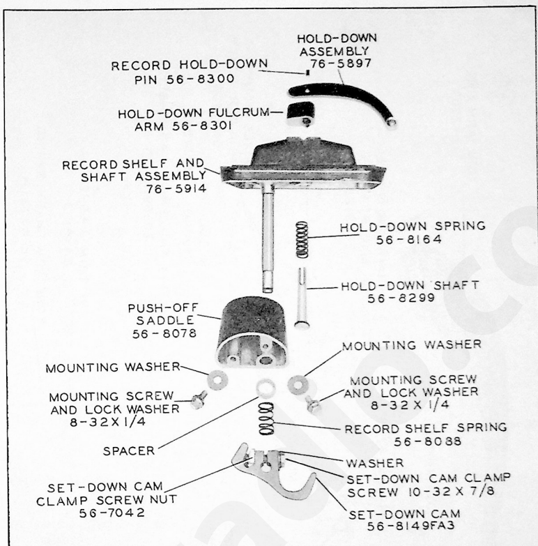
Figure 14. Record-Shelf Assembly
