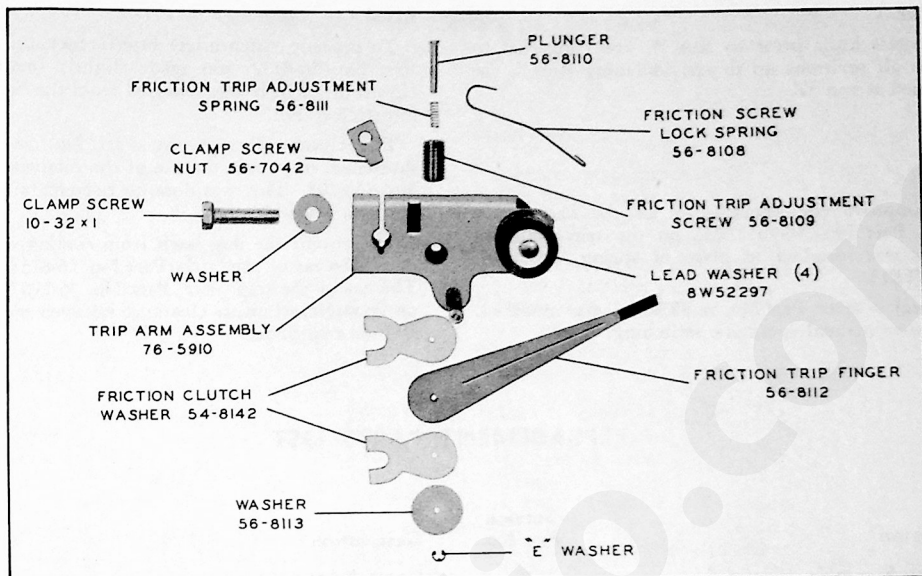
Figure 16. Trip-Arm Assembly
