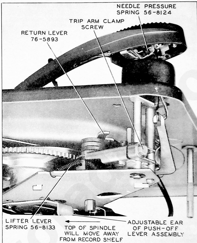
Figure 3. Adjustment of Trip Arm for 7" Set-down
